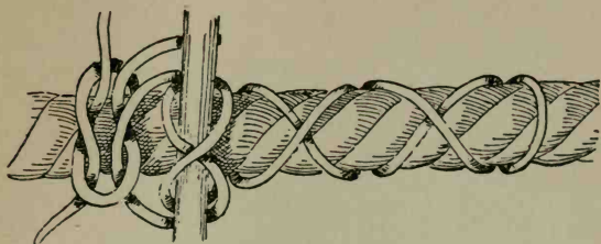
FIG. 47.—Chain hitch with bar.
